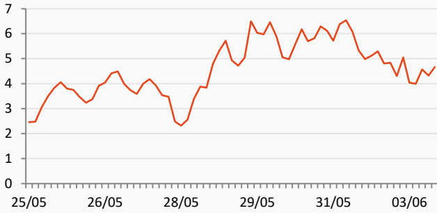
Power Forward Contracts Baseload £/MWh
